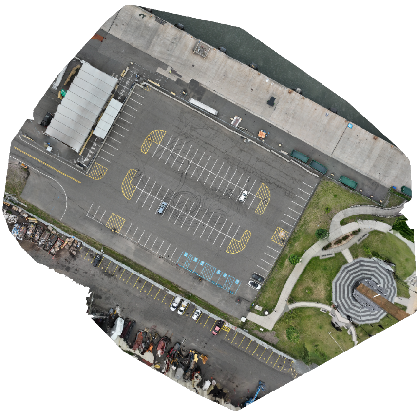
Orthophoto
